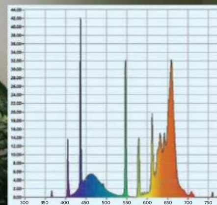
Marigold's Induction Lamp
